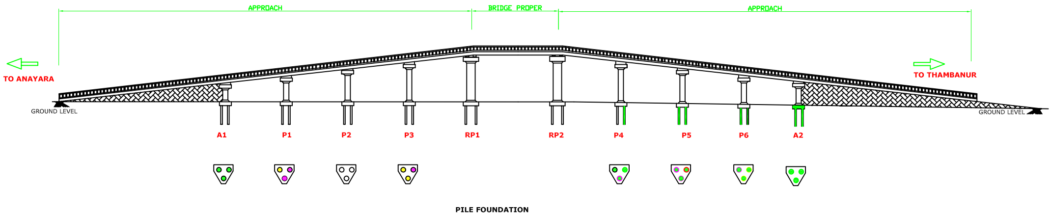
PILE FOUNDATION
